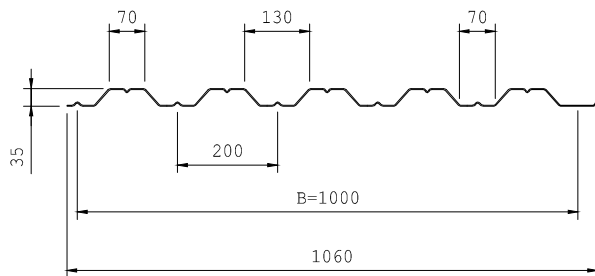
DF HC35-1000
