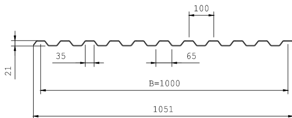
DF C21-1000
